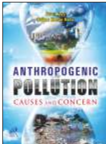
Anthropogenic Pollution
