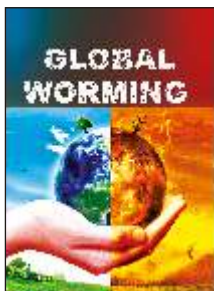
Global Warming
